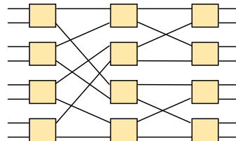
Flip network (inverse shuffle exchange)
