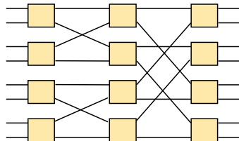
Shuffle exchange (Omega) network
