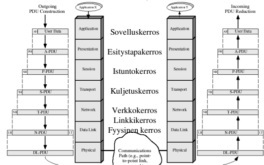
Figure 2.6 The OSI Environment
