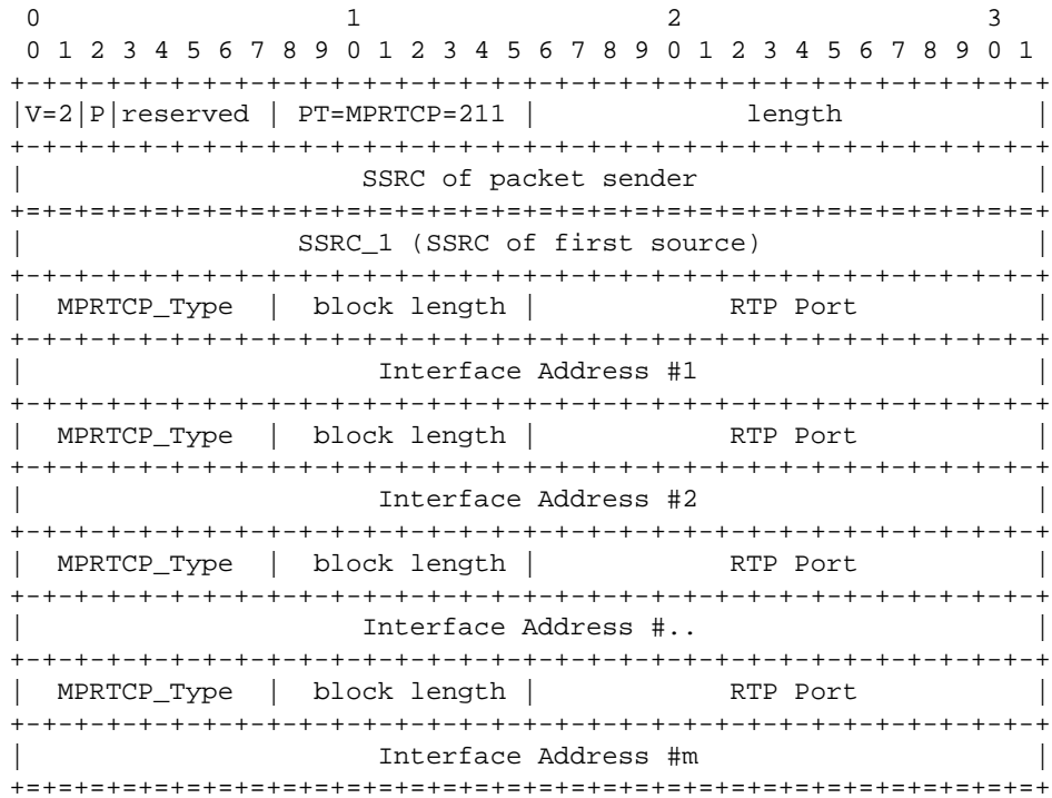
Figure 13: MPRTCP Interface Advertisement. (appended to SR/RR)
