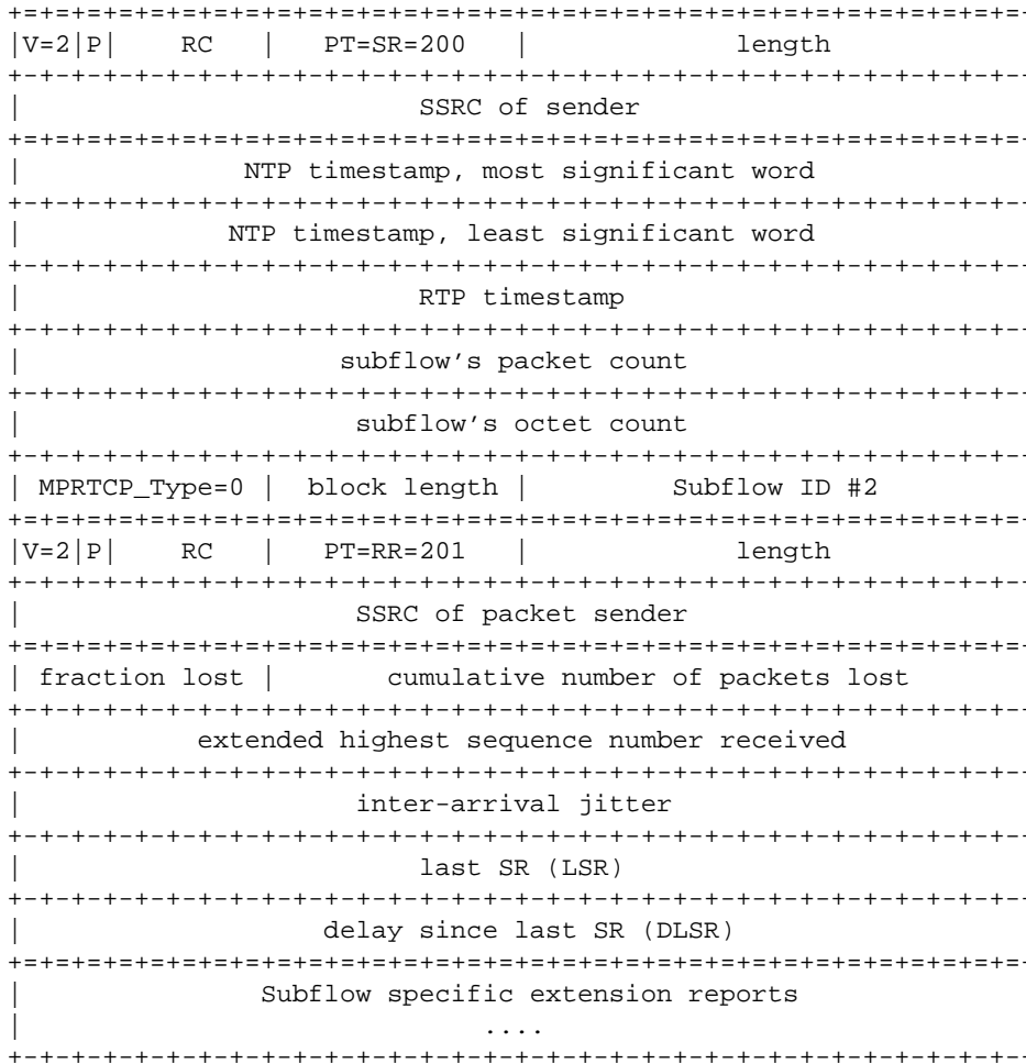
Figure 12: Example of reusing RTCP SR and RR inside an MPRTCP header (Bi-directional use-case, in case of uni-directional flow the subflow will only send an SR or RR).
