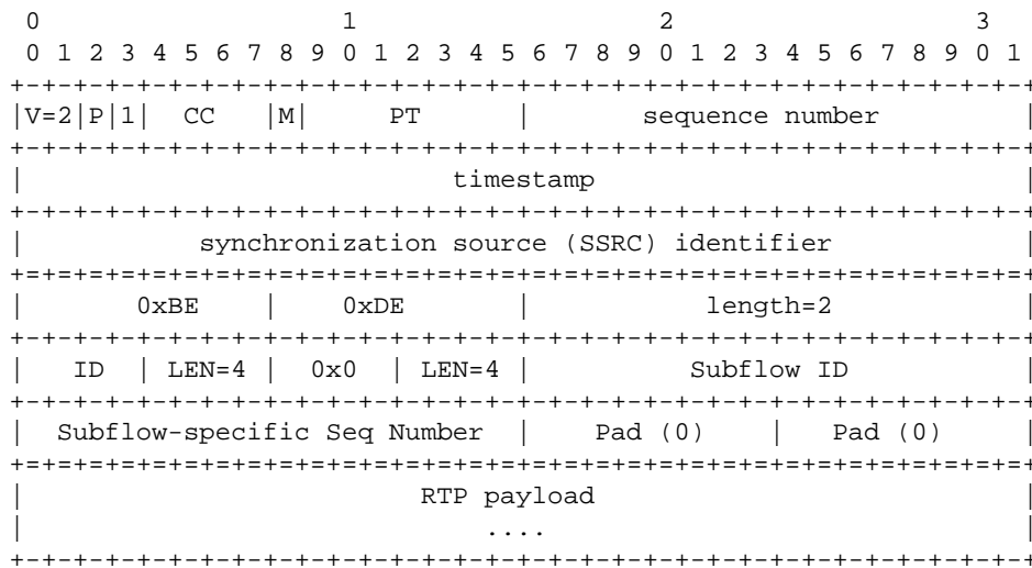
Figure 8: MPRTP header for subflow
