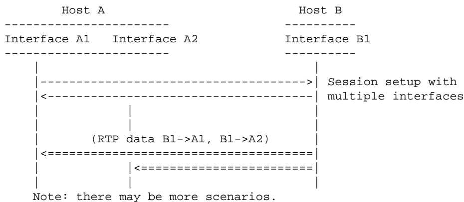
Figure 3: Unidirectional media flow
