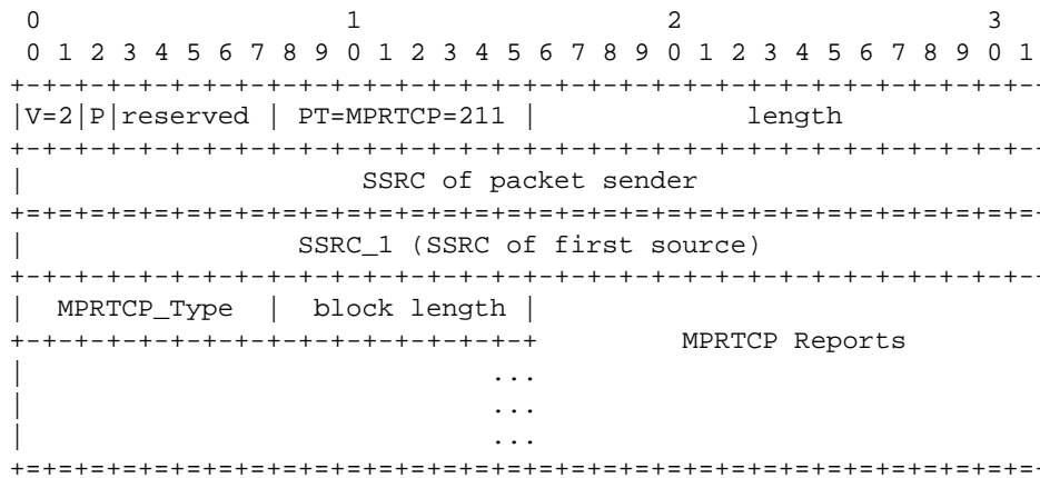
Figure 9: Generic RTCP Extension for MPRTCP (MPRTCP) [appended to normal SR/RR]
