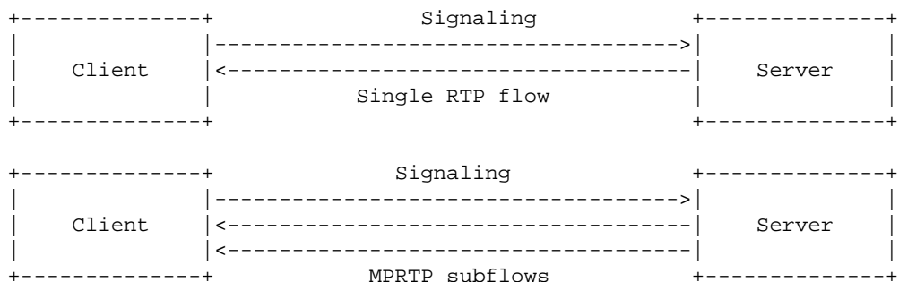
Figure 1: Comparison between traditional RTP streaming and MPRTP
