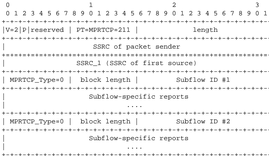
Figure 11: MPRTCP Subflow Reporting Header
