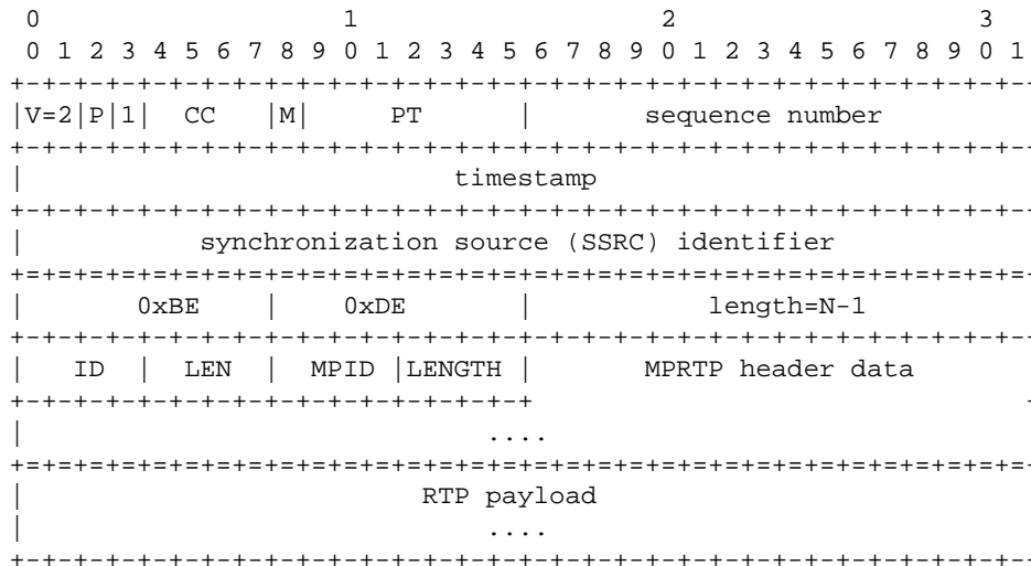
Figure 6: Generic MPRTTP header extension
