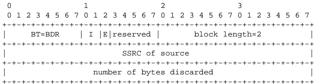
Figure 2: XR Bytes Discarded Report Block
