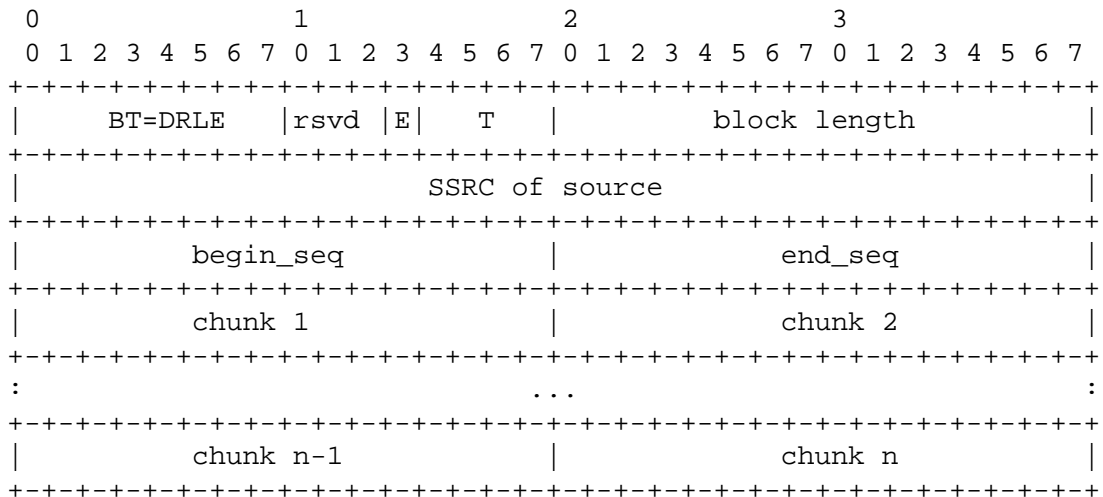
Figure 1: XR Discard Report Block
