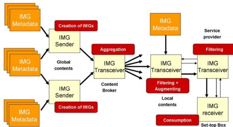
Figure 2: Sample IMG Operation with Metadata Aggregation and Personalisation
