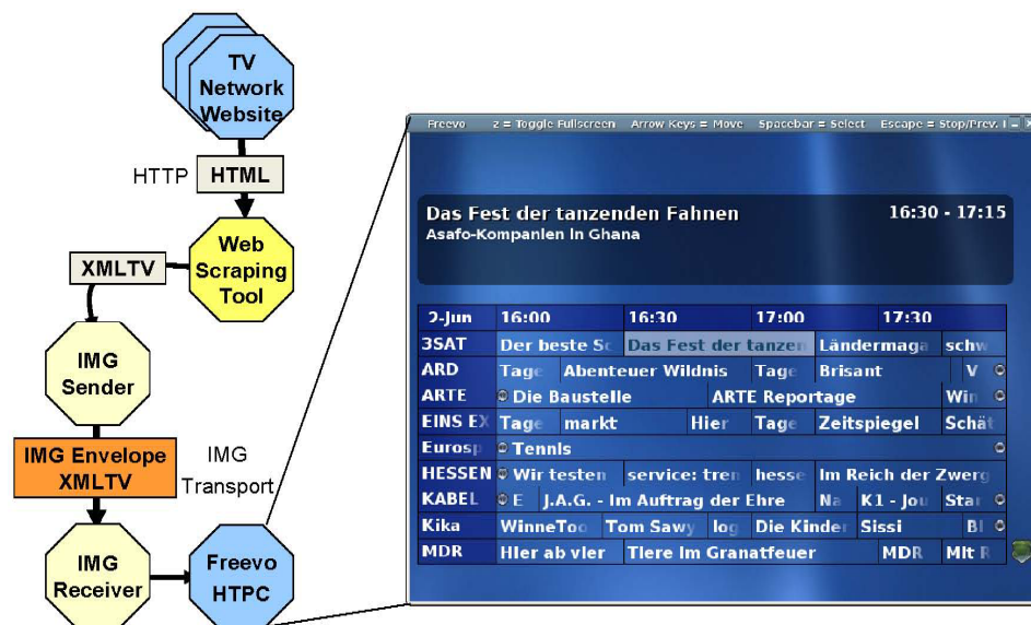
Figure 5: TV-EPG distribution
