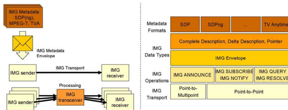
Figure 1: Architecture Overview
