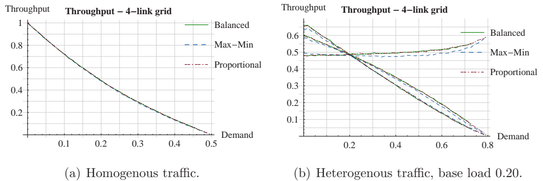
Figure 6.8: Throughput in 2 \times 2 grid.
