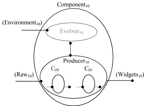
Figure 8: Atomic Components
