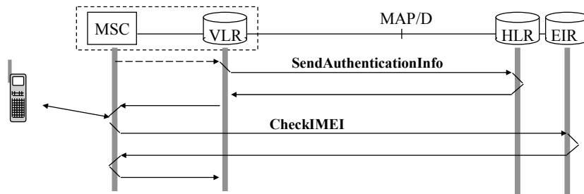
Figure 9.15 Security operations for circuit switched services
