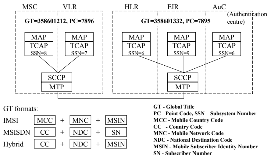
Figure 9.9: Addressing in MAP
