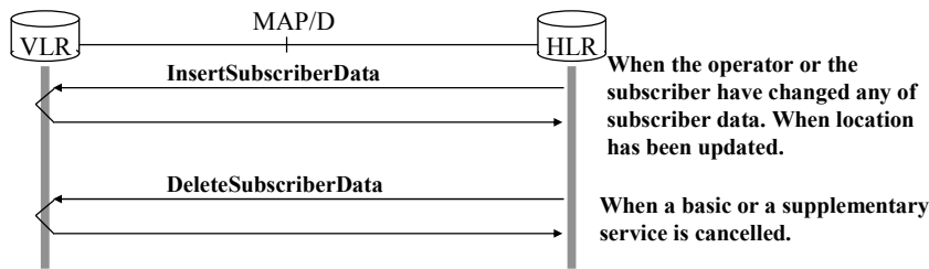
Figure 9.16: Subscriber management operations
