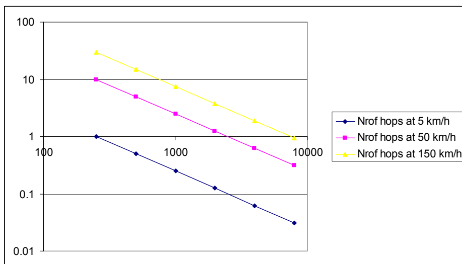
Figure 9.3: Number of cell hops at speed of 5, 50 and 150 km/h as a function of cell diameter.
