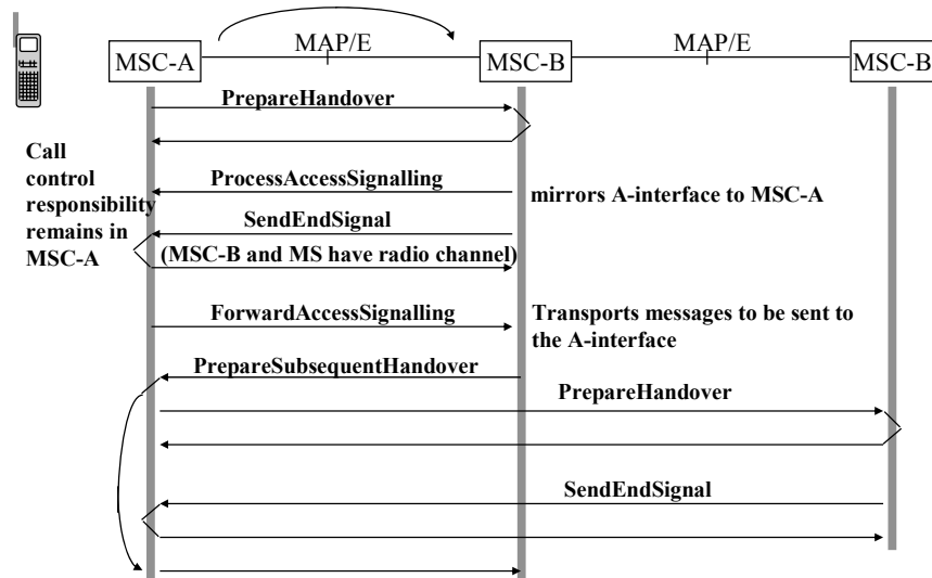
Figure 9.14: MAP support for MSC to MSC handover.
