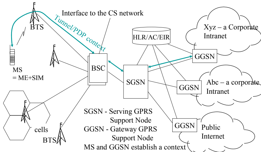
Figure 9.4: GPRS network.
