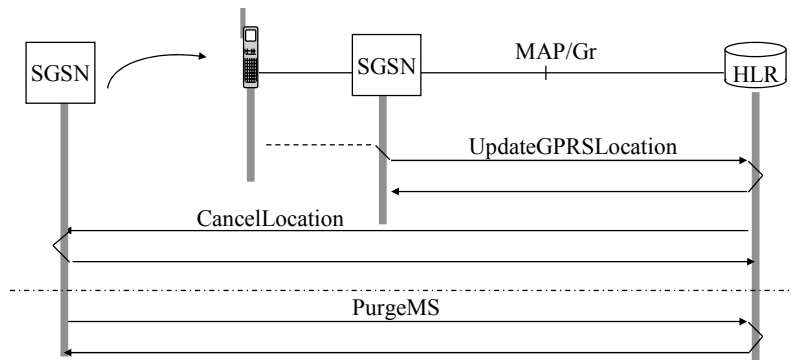
Figure 9.12: MAP operations for packet terminal location management
