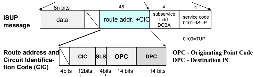
Figure 6.1 Message routing information in ISUP and MTP
