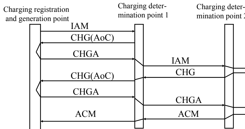
Figure 6.4: Charging support in ISUP.
