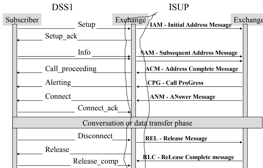
Figure 6.3: Interworking of DSS1 and ISUP for Successful call setup
