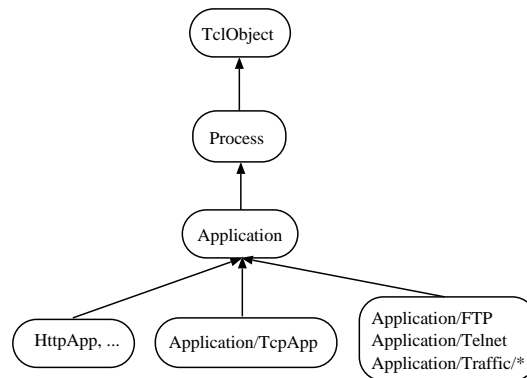
Figure 36.2: Hierarchy of classes related to application-level data handling
