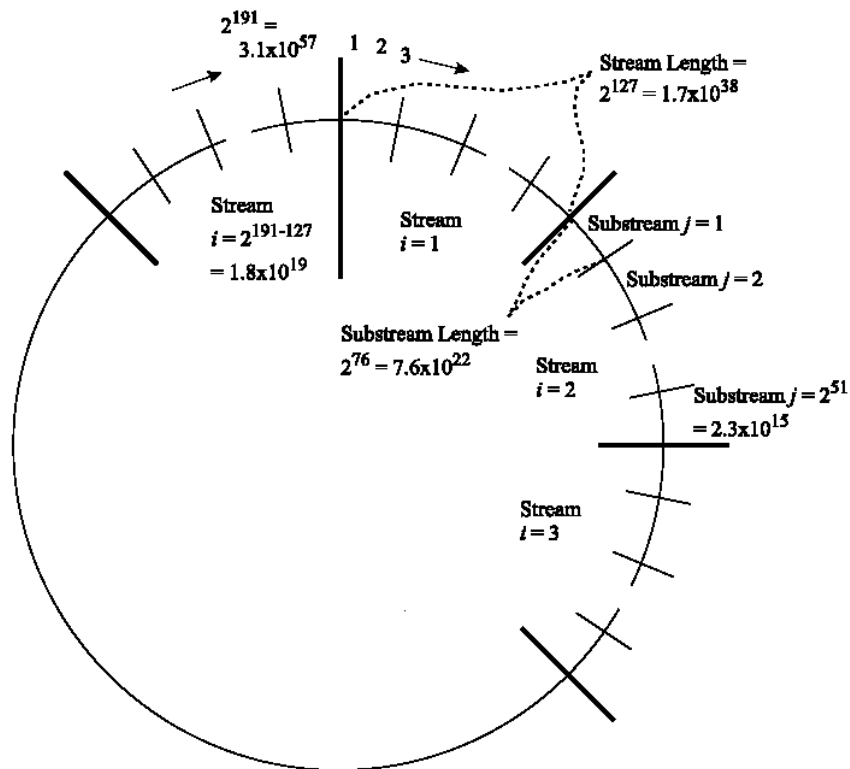
Figure 22.1: Overall arrangement of streams and substreams. [19]
