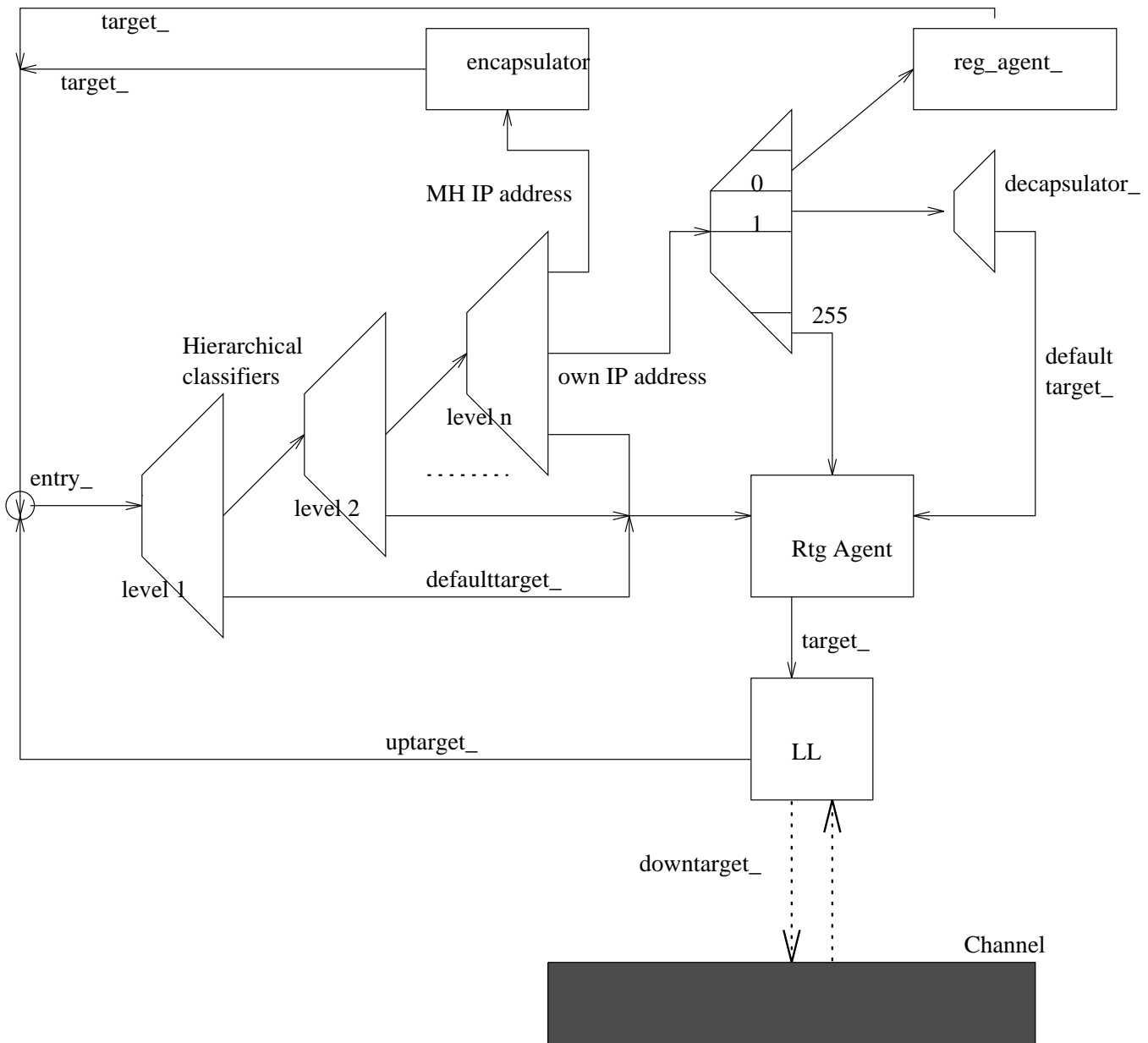
Figure 16.4: Schematic of a Wireless MobileIP Base Station Node
